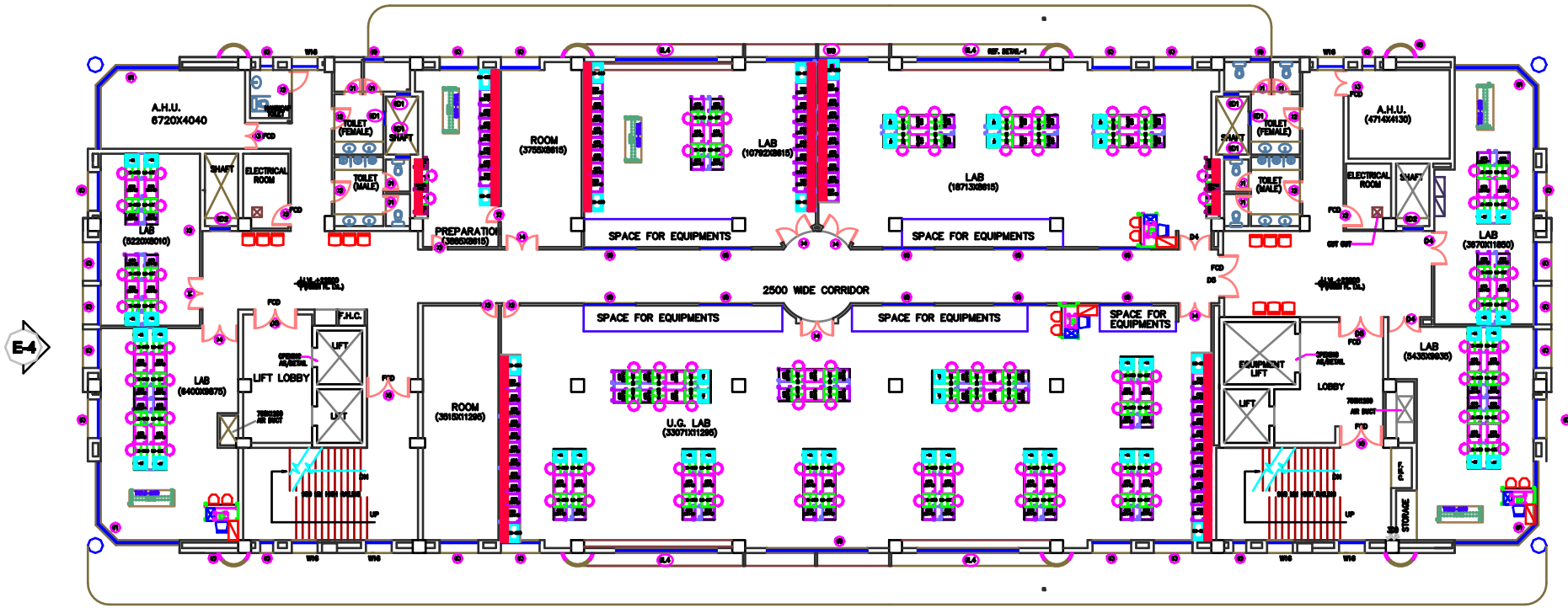
6TH FLOOR PLAN
